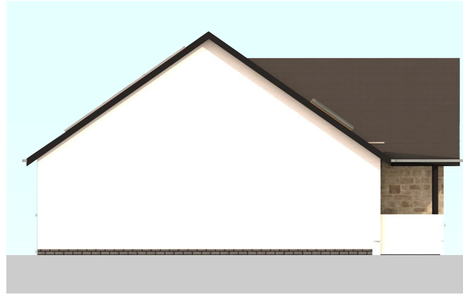
Side 1 Elevation
